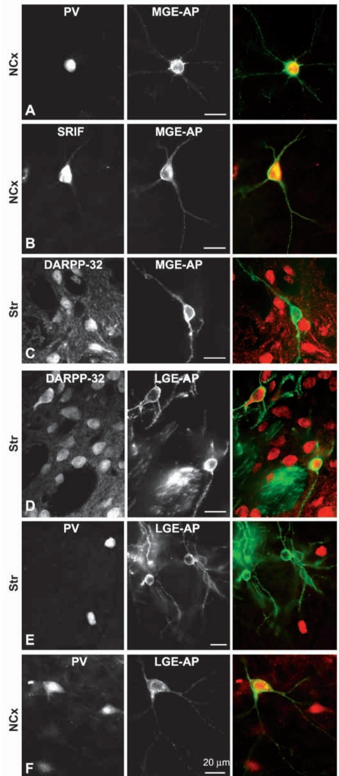
Fig. 5. Immunohistochemical characterization of grafted MGE (A-C) and LGE (D-F) cells in the neocortex (NCx; A,B,F) and striatum (Str; C,D,E). MGE-derived cells are from a 4-month-old animal, LGE-derived cells are from 3-week-old animal. The second column and green color in the third column represent staining for alkaline phosphatase expressed in transplanted cells. (A-C) Many MGE cell in the neocortex expressed parvalbumin (A) and somatostatin (B) but within striatum did not express striatal marker DARPP-32 (C). (D,E) The majority of LGE cells in the striatum expressed DARPP-32 (D) but did not express parvalbumin (E). (F) By contrast, some of the LGE-derived neurons that migrated into the neocortex expressed parvalbumin.
